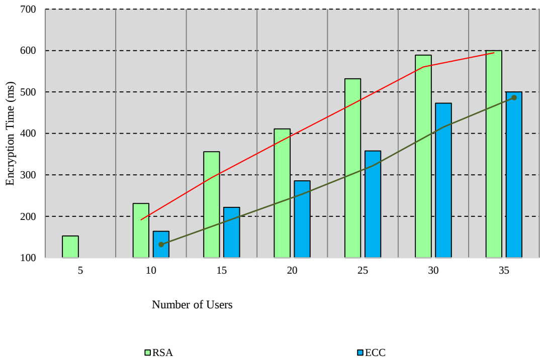
Fig.2. Decryption Time vs. Number of Users
