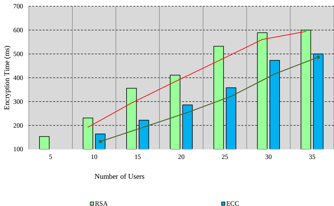
Encryption Time vs. Number of Users
