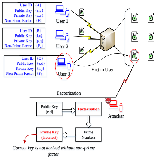
Fig.4. Attacks in ECC
