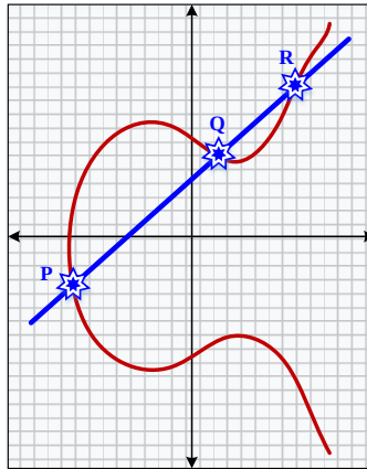
Fig.1. Elliptic curve
